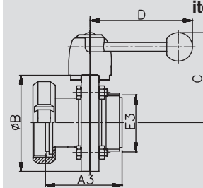
butterfly valve SV04 IDF LM handle HB04 item-no. 56544-
